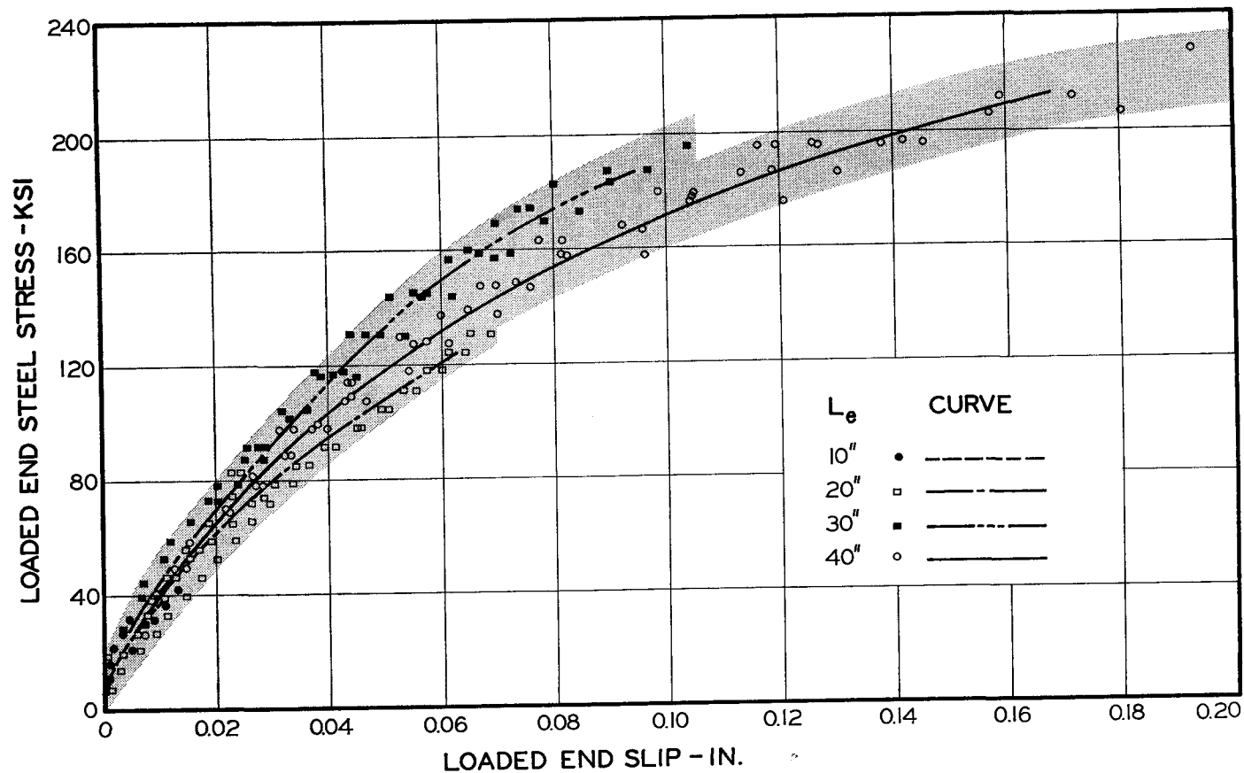
Fig. 6. Slip as a function of loaded end steel stress for the four embedment lengths of the bent series.
