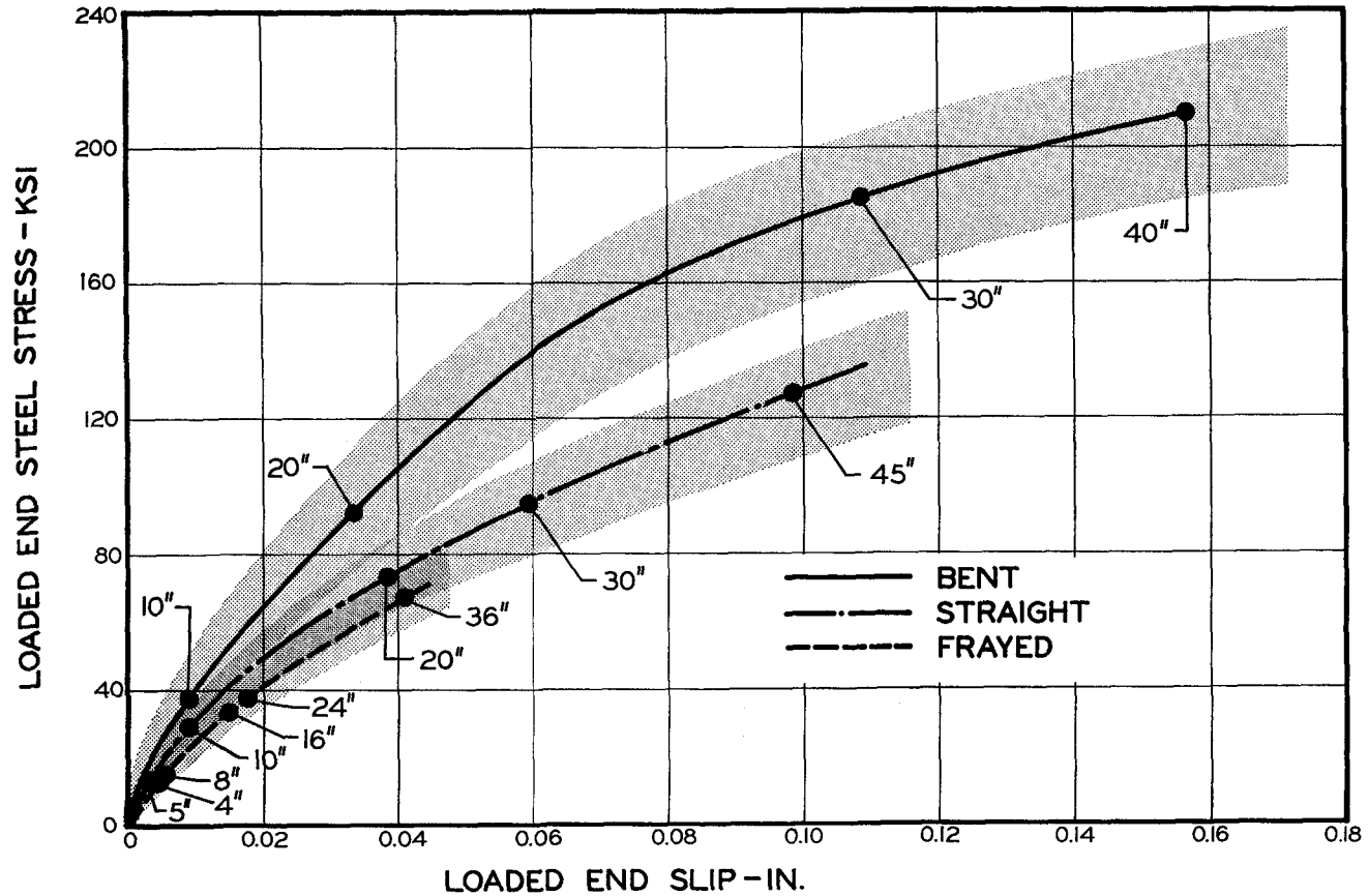
Fig. 7. Steel stress versus loaded end slip for the three strand configurations.
