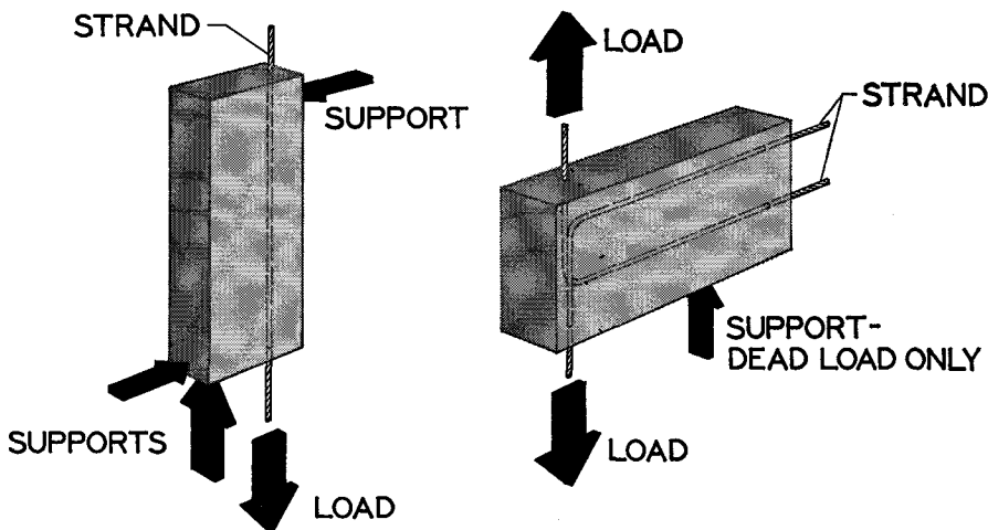
Fig. 1. Specimen configuration: (left) straight strand; (right) bent strand.
