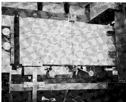
Fig. 4. Bent strand specimen during testing.
